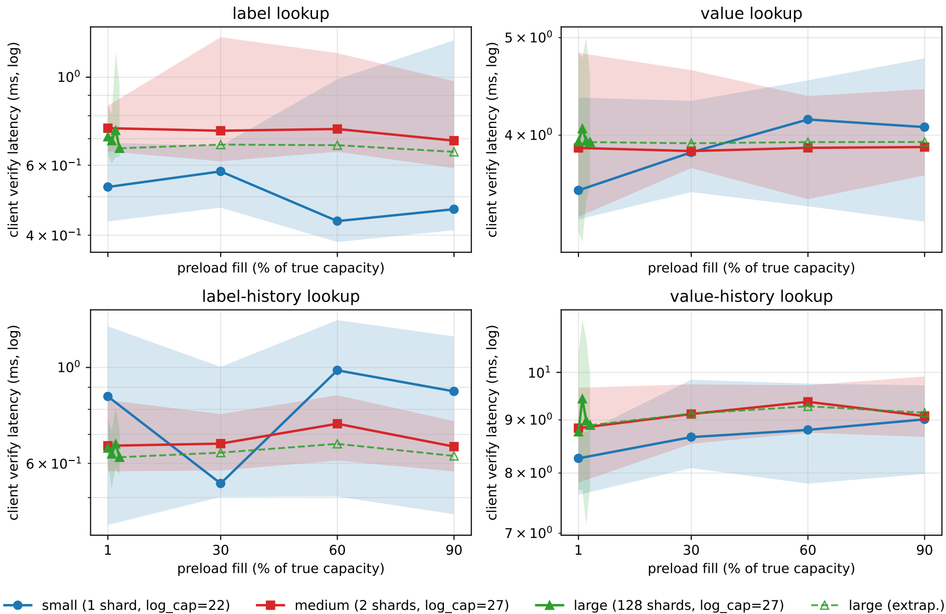
Client-side lookup verify latency vs. preload (median, shaded = 10th-90th percentile; dashed = extrapolation)
