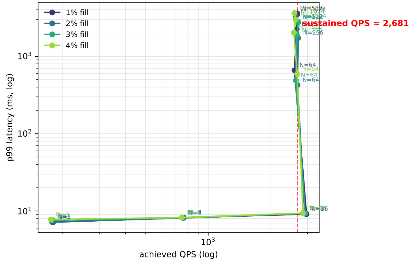
Latency knee — large regime (p99 vs. QPS, value RPC; one curve per fill level)
