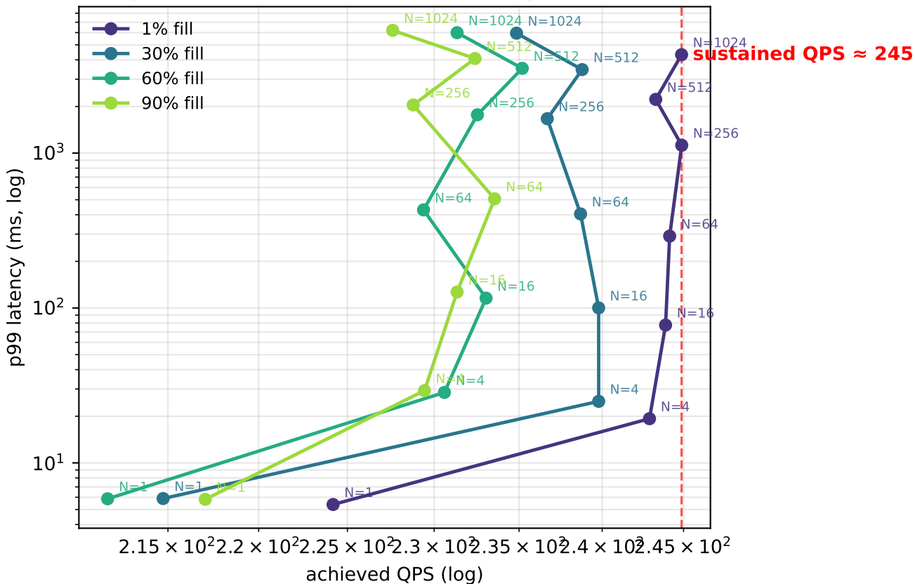
Latency knee — small regime (p99 vs. QPS, value RPC; one curve per fill level)
