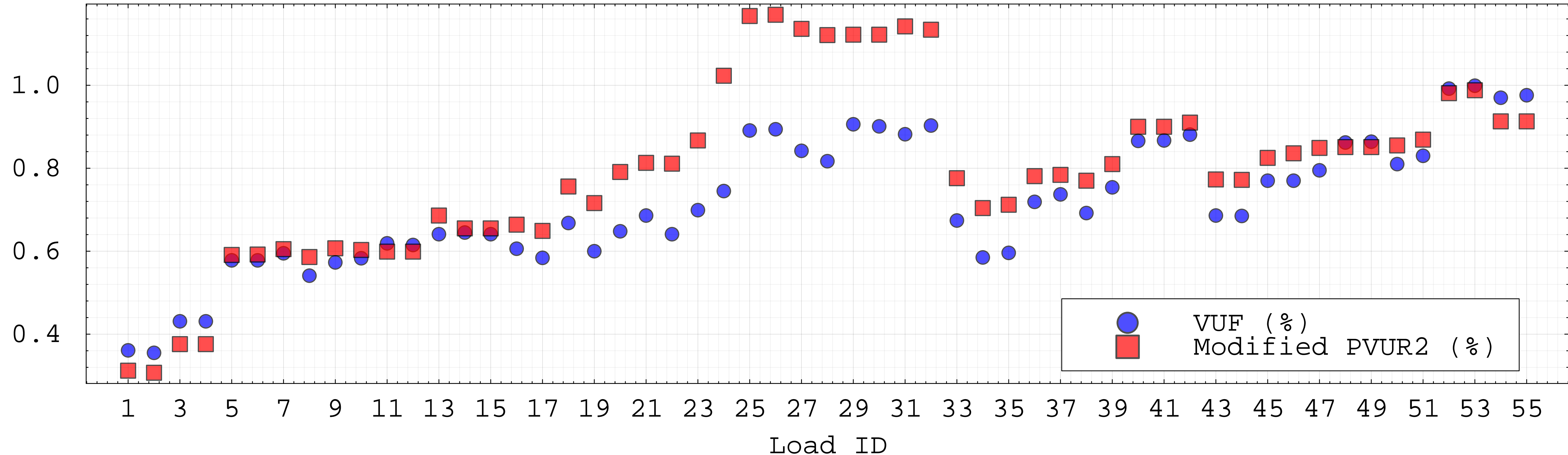
Voltage Unbalance (%)
