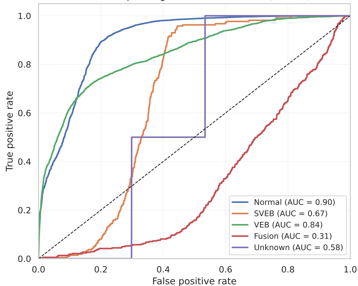
Receiver operating characteristic curves (test set)
