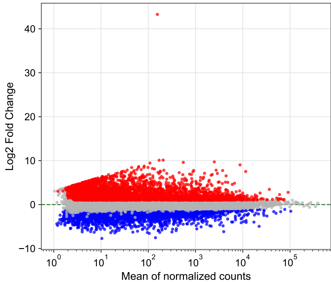
MA Plot - TCGA-Project
