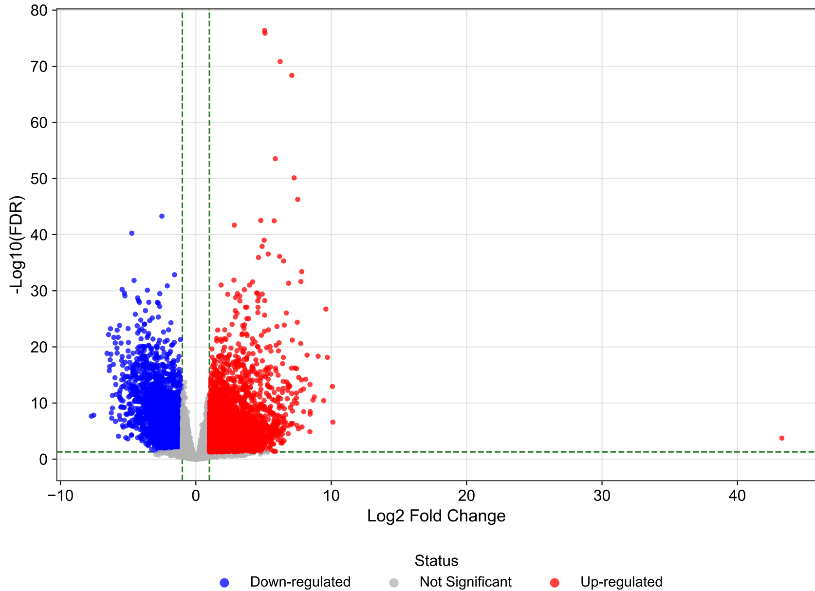
Volcano Plot - TCGA-Project (Tumor vs Normal)
