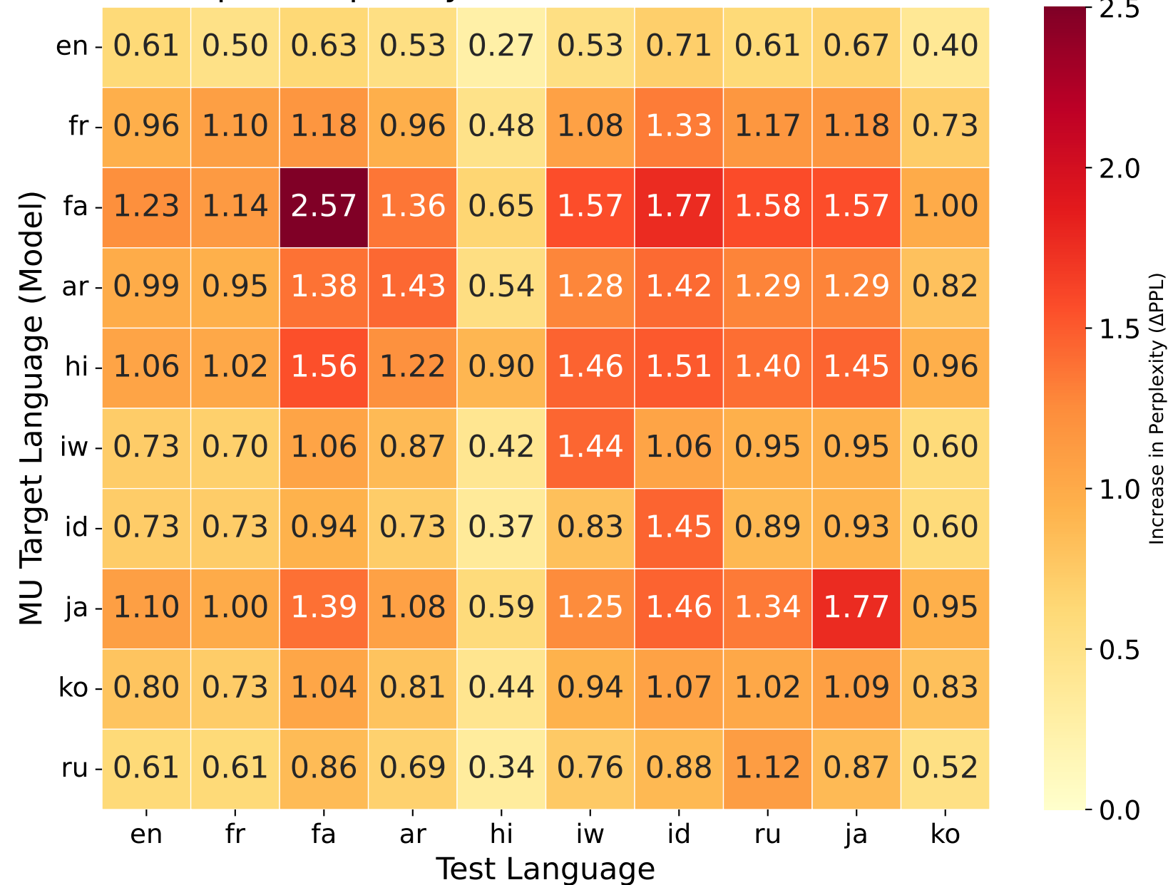
Heatmap of Perplexity Increase ( \Delta PPL) vs. Base Model
