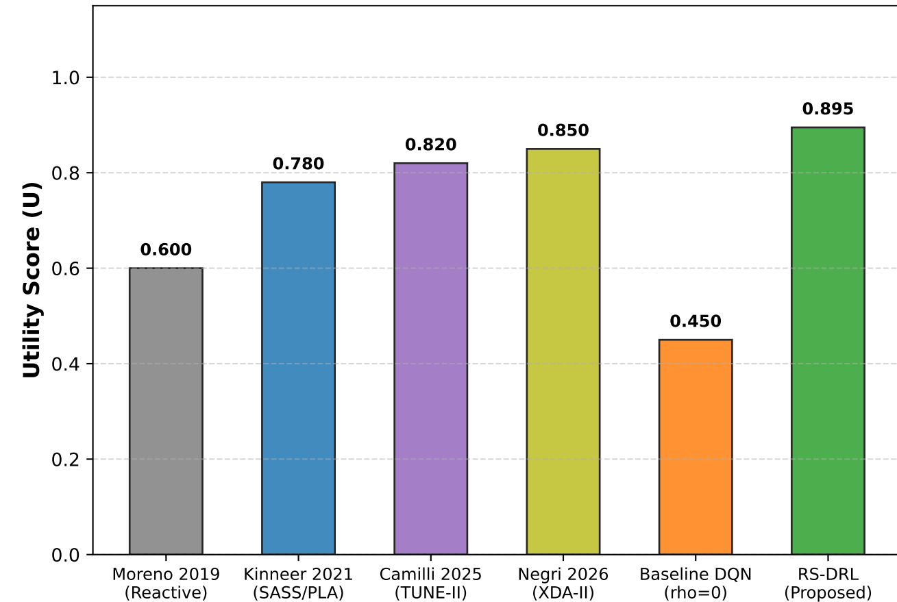
(d) Overall Multi-Objective Utility Score
