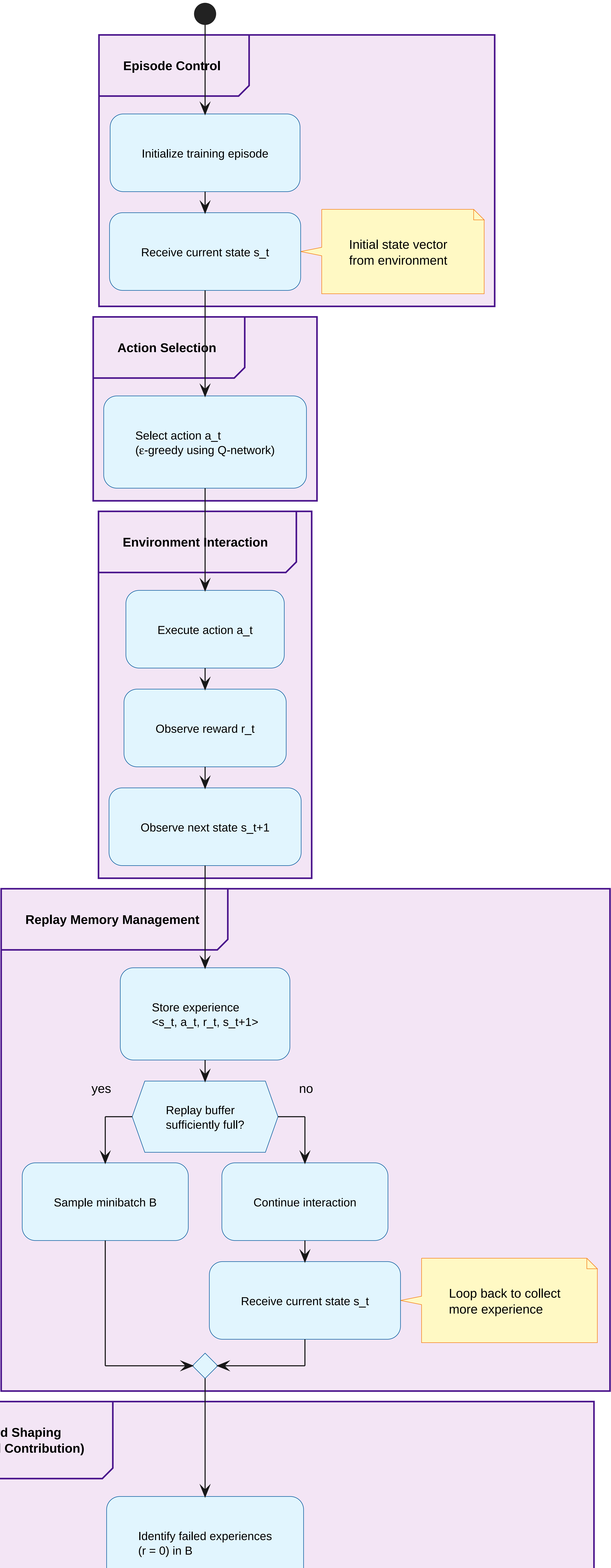
RS-DRL Training & Reward Shaping Process (UML Activity Diagram - Deep Dive)
