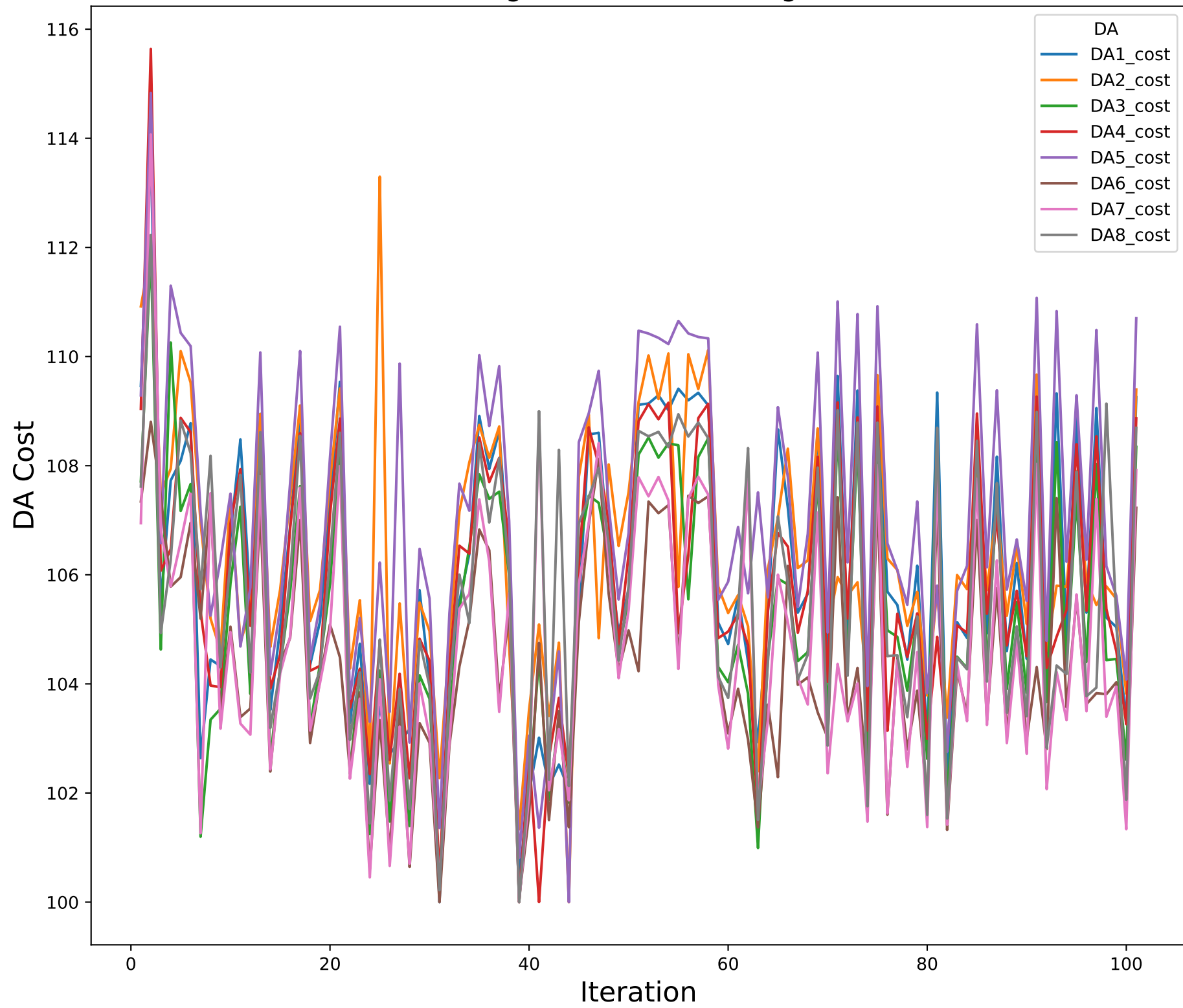
(a) Diagonalization Convergence
