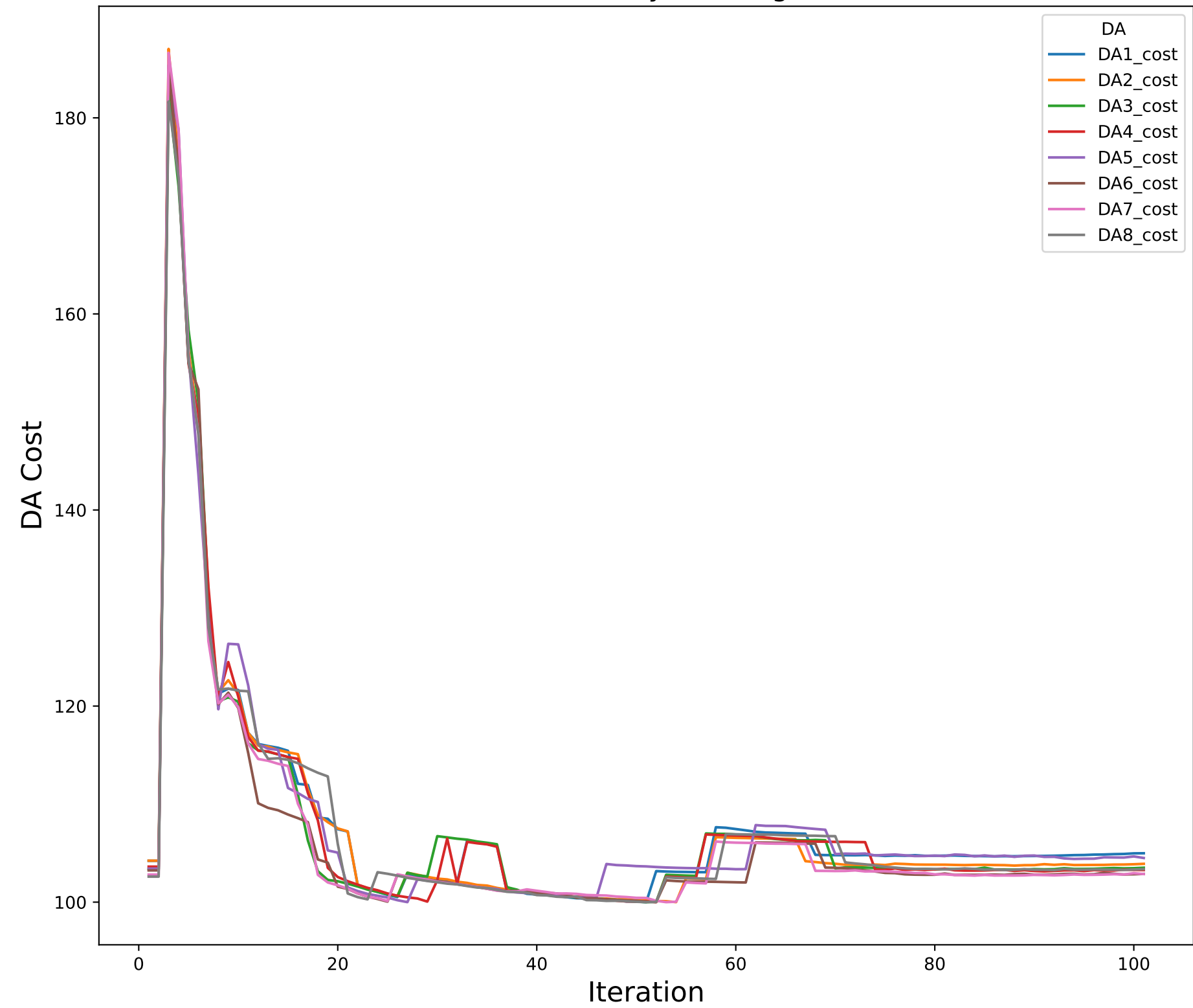
(b) FictitiousPlay Convergence
