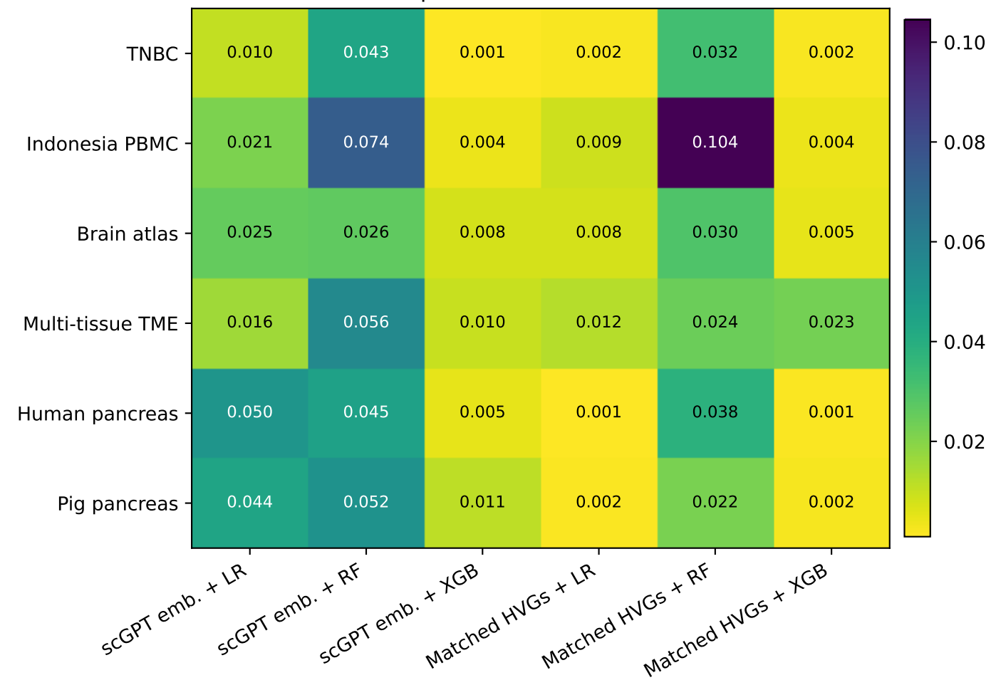
Expected calibration error
