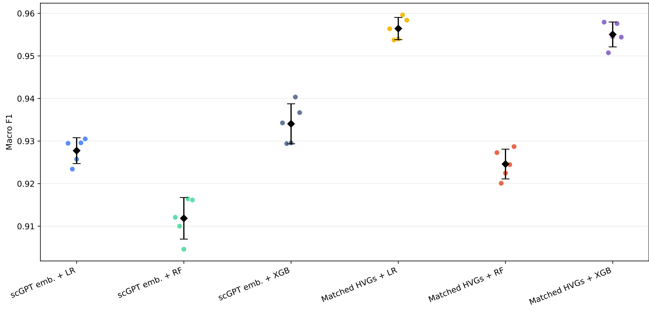
Five donor-held-out folds on Indonesia PBMC
