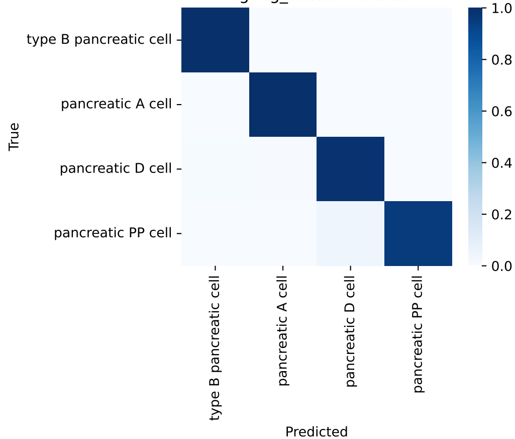
LogReg_vocab-matched
