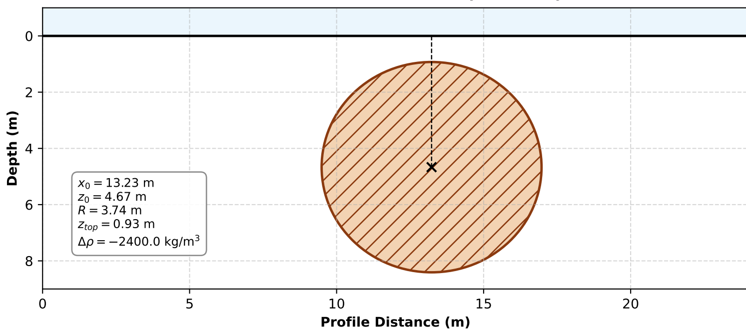
(c) Inverted Subsurface Cavity Geometry
