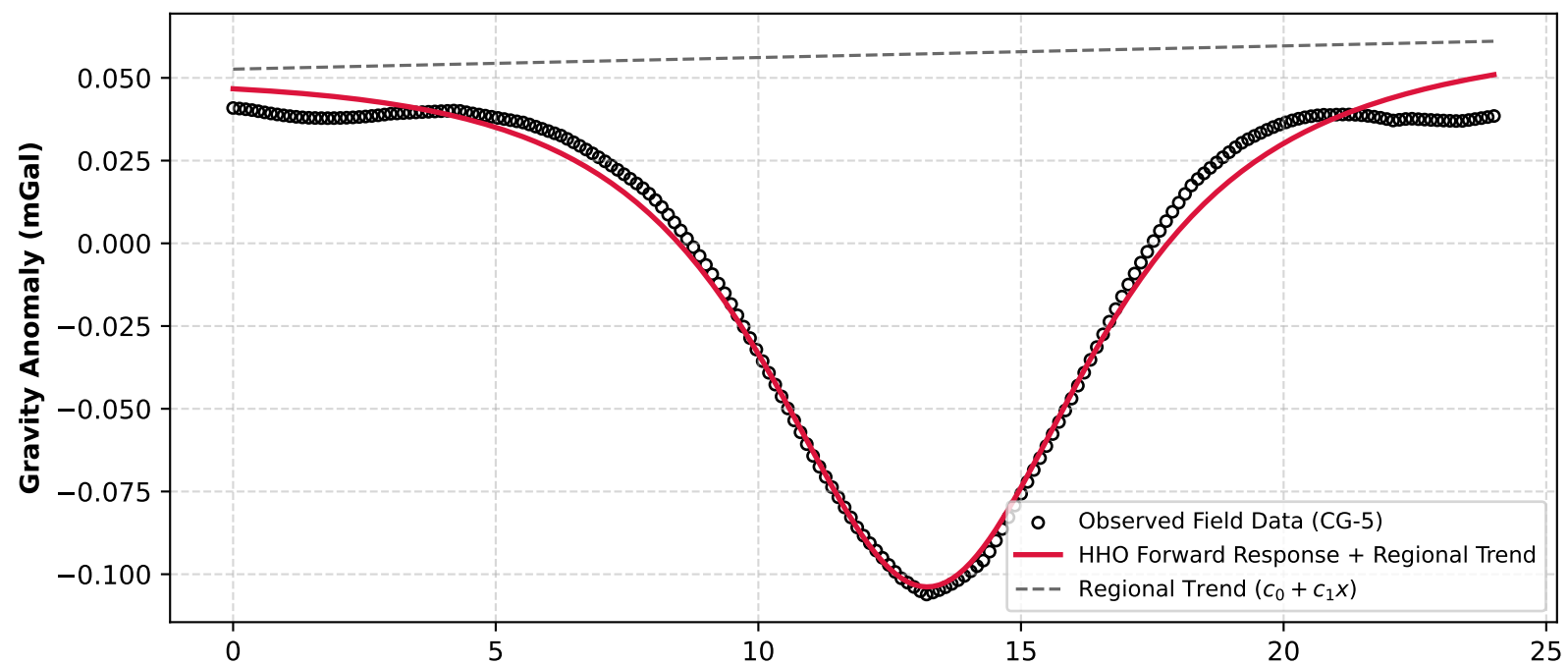
(a) Field Gravity Anomaly and Inversion Model Fit
