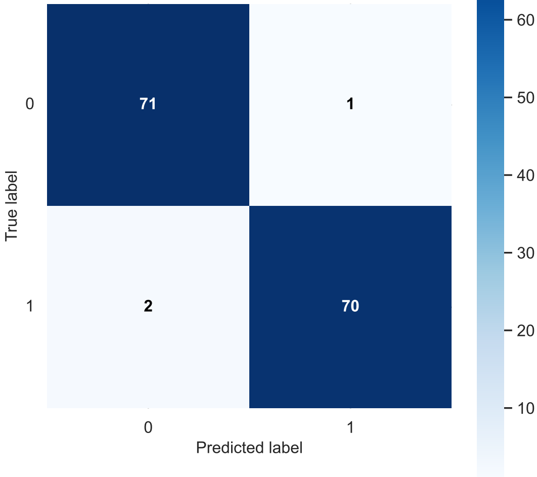
Confusion Matrix Subject 1
