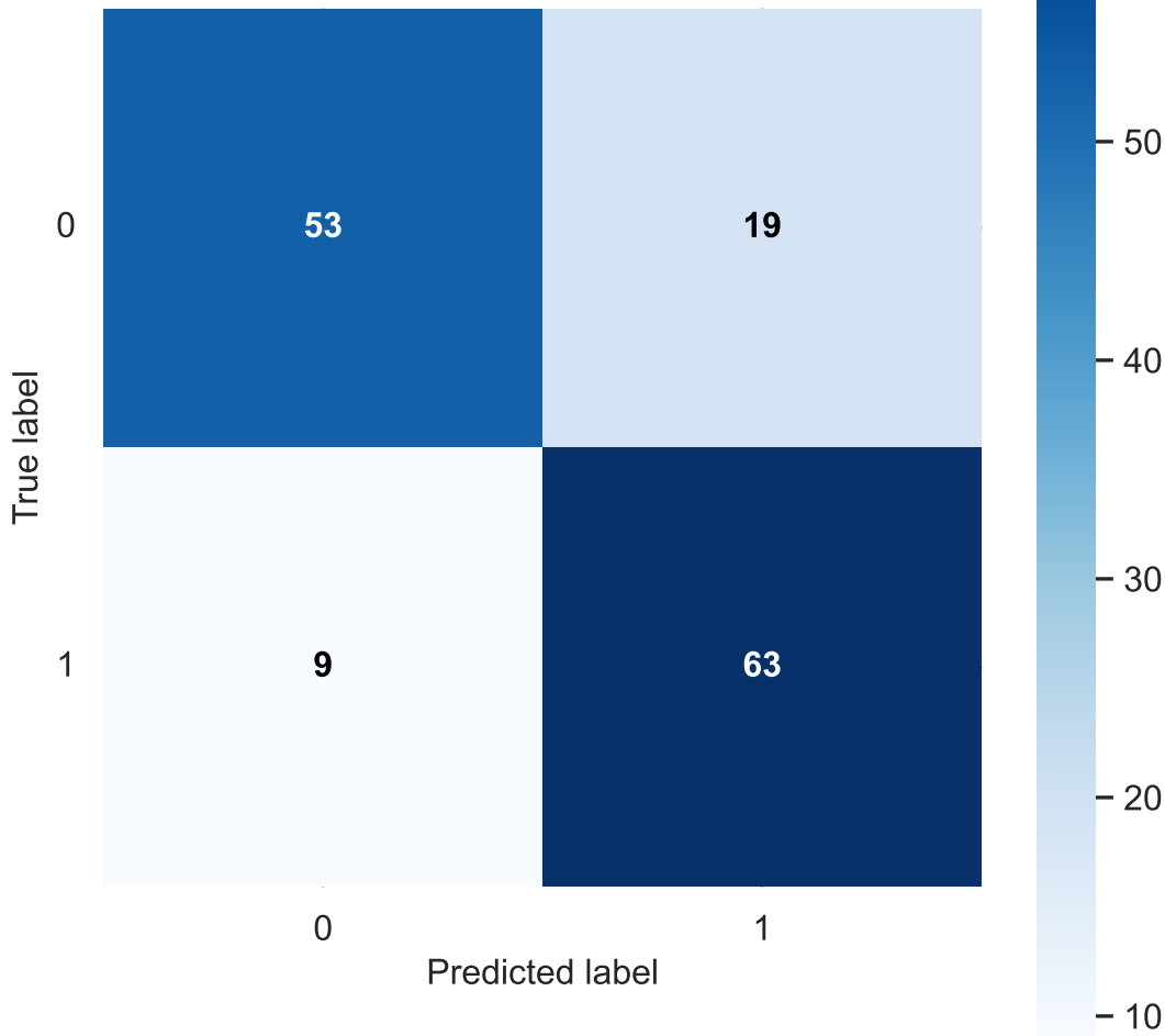
Confusion Matrix Subject 2
