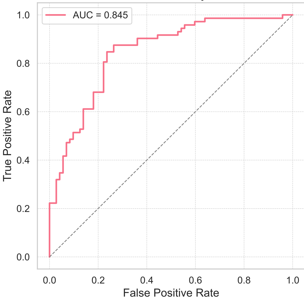
ROC Curve Subject 2
