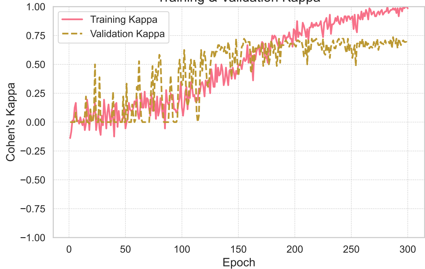
Training & Validation Kappa
