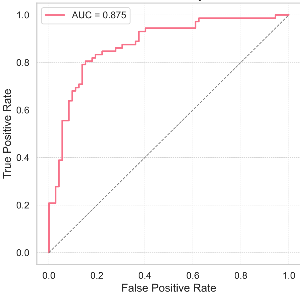
ROC Curve Subject 7
