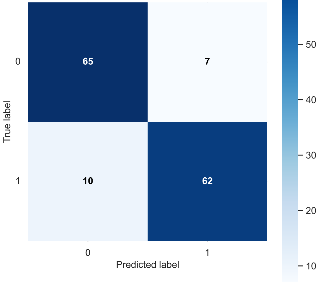
Confusion Matrix Subject 8
