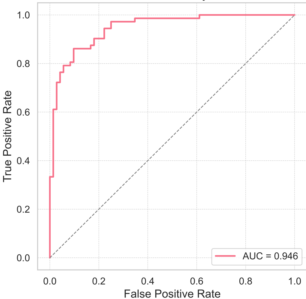
ROC Curve Subject 8
