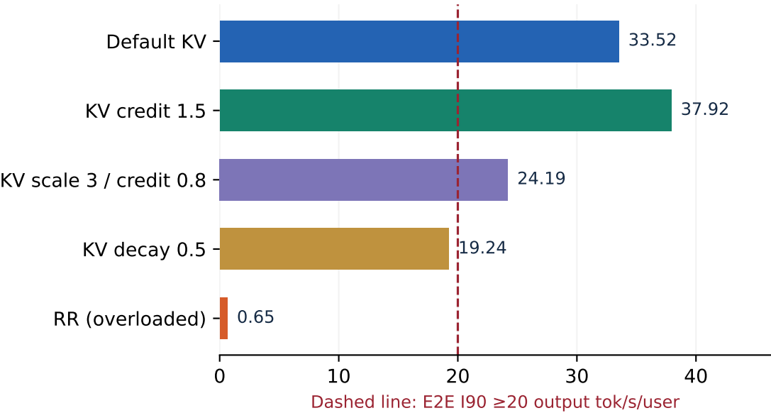
E2E I90 (output tok/s/user; higher is better)
