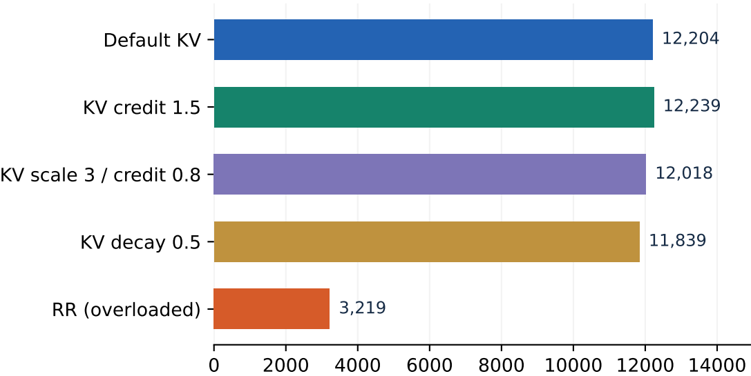
Total input + output tokens/s/GPU
