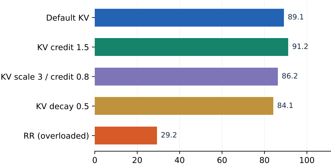
Frontend-reported cached input (%)
