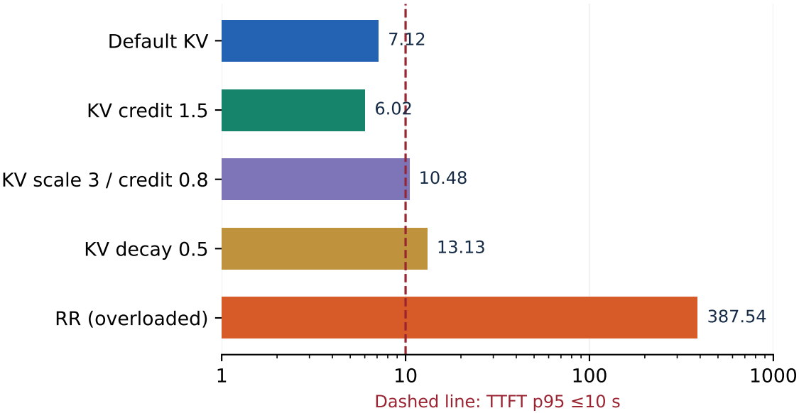
TTFT p95 (seconds; lower is better)
