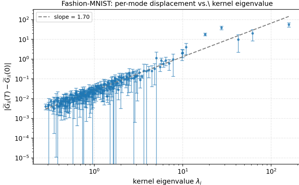
Figure 6: Spectral-bias prediction on Fashion-MNIST. Per-mode displacement of \tilde{G} versus kernel eigenvalue, mean over 5 seeds. The same mode-wise rate ordering appears as in the synthetic case.
