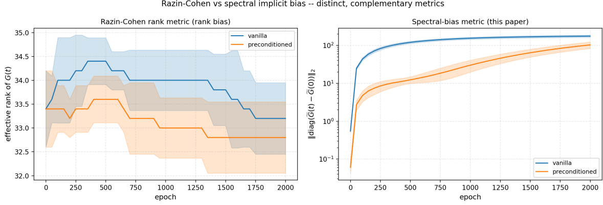
Figure 9: The kBM spectral implicit bias is distinct from the Razin–Cohen rank bias. Left: effective-rank trajectory of G(t) (the Razin–Cohen metric) is trivial and indistinguishable across methods. Right: spectral-displacement trajectory (this paper, log scale) shows large vanilla deviation from initialization that the preconditioner suppresses. Our mechanism operates along K ’s eigenbasis, not along the rank dimension.
