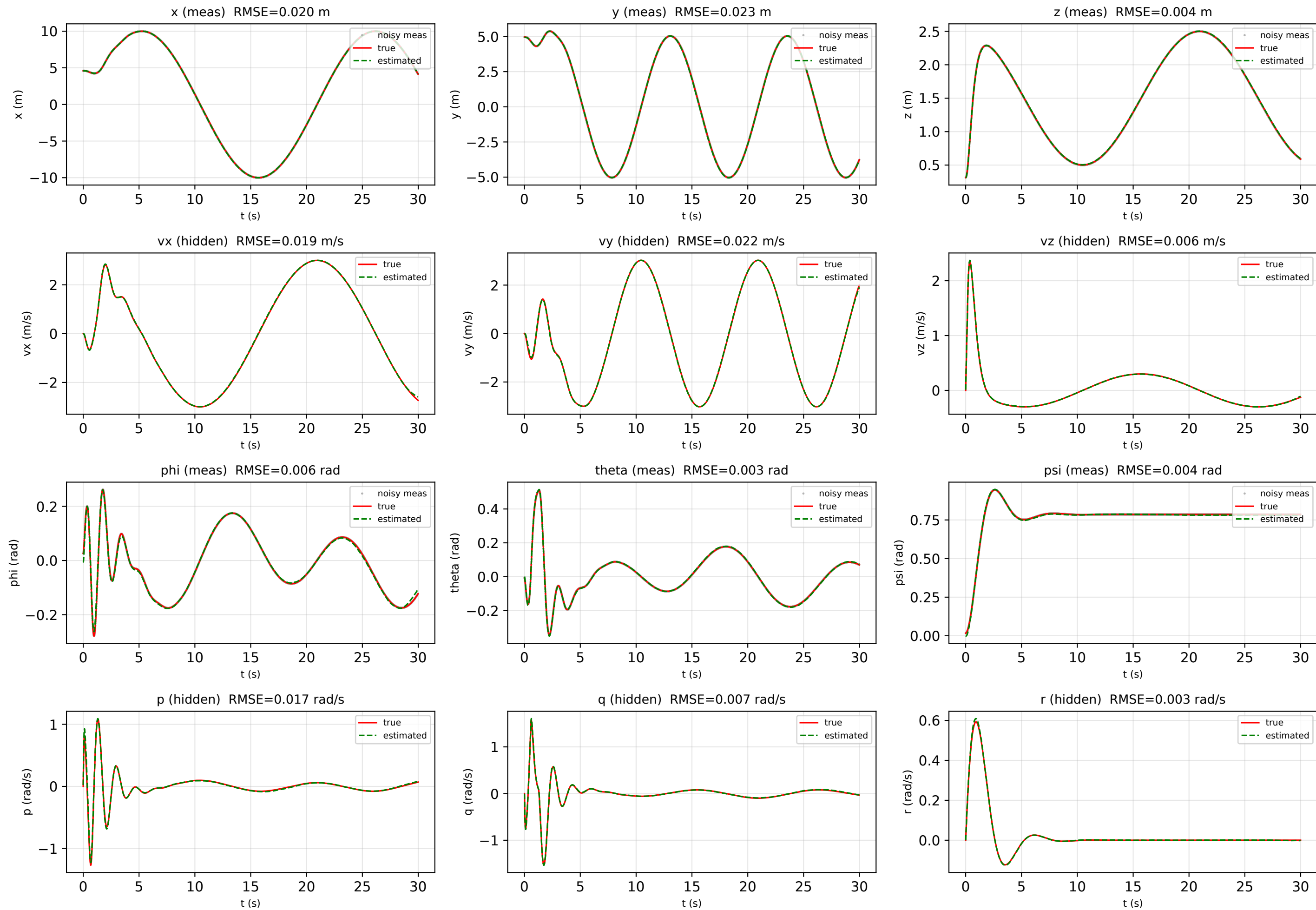
Figure-eight: PINN observer on an unseen flight -- true vs estimated (all 12 states)
