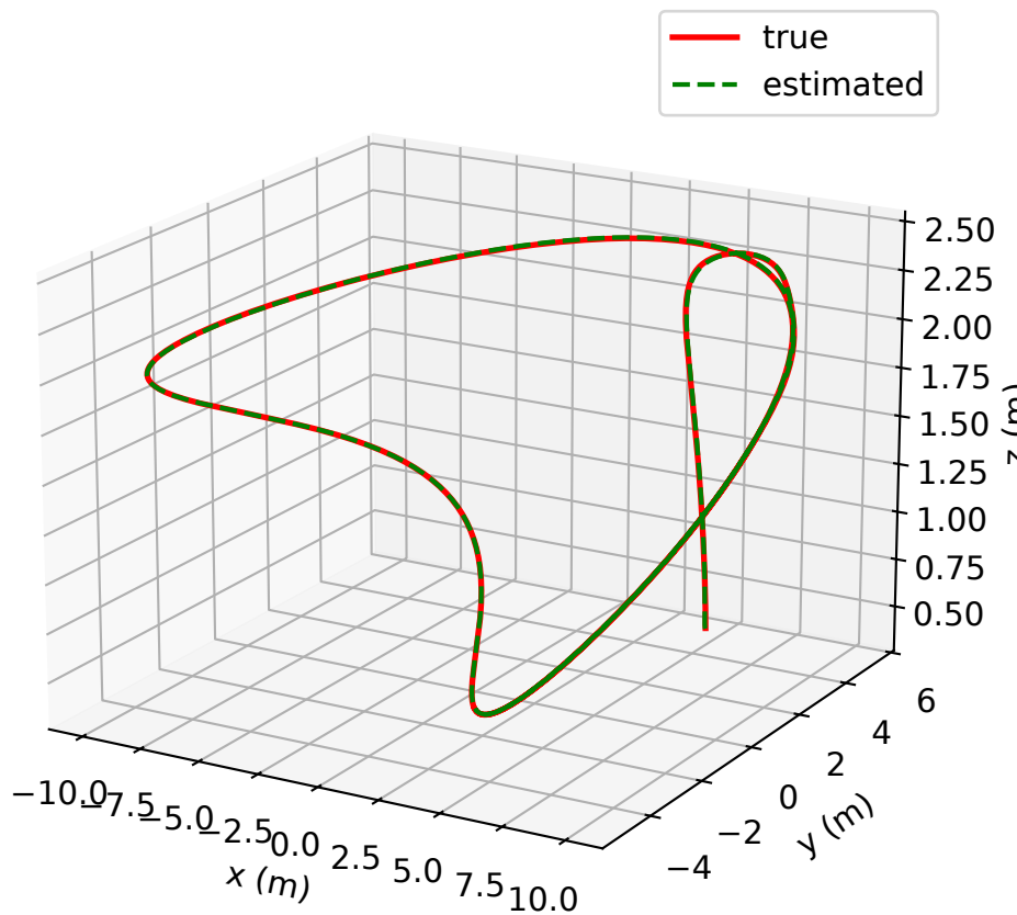
Figure-eight: PINN observer, true vs estimated (3-D)
