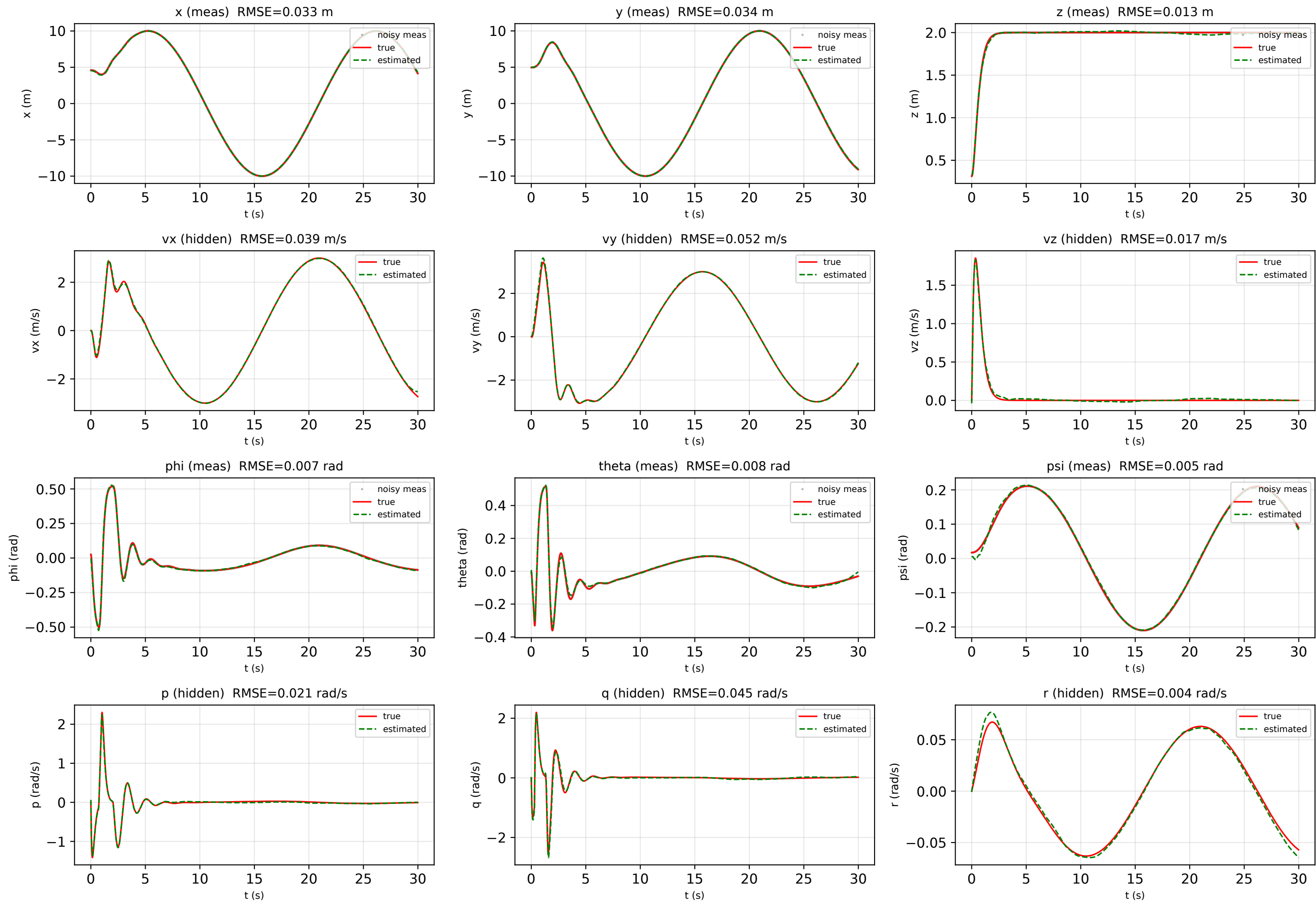
Circle: PINN observer on an unseen flight -- true vs estimated (all 12 states)
