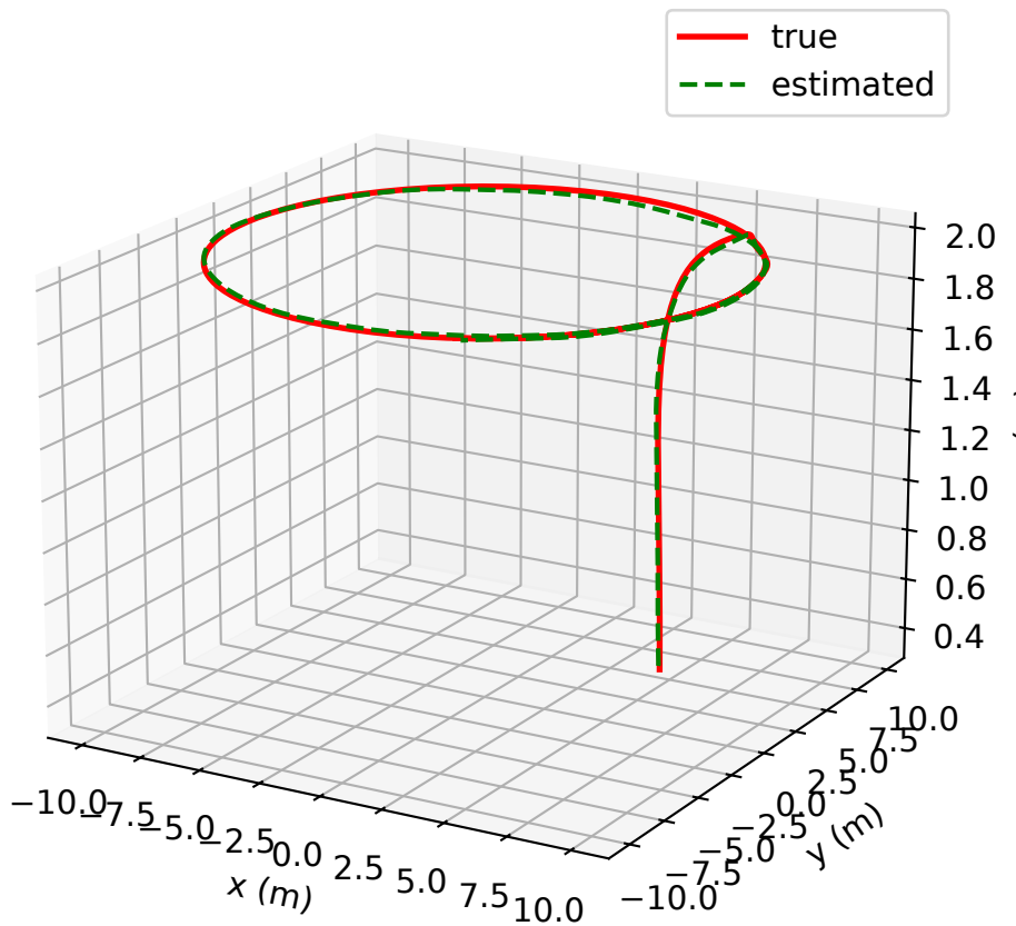
Circle: PINN observer, true vs estimated (3-D)
