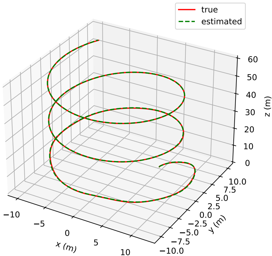
PINN observer - 3D trajectory position RMSE=0.115 m
