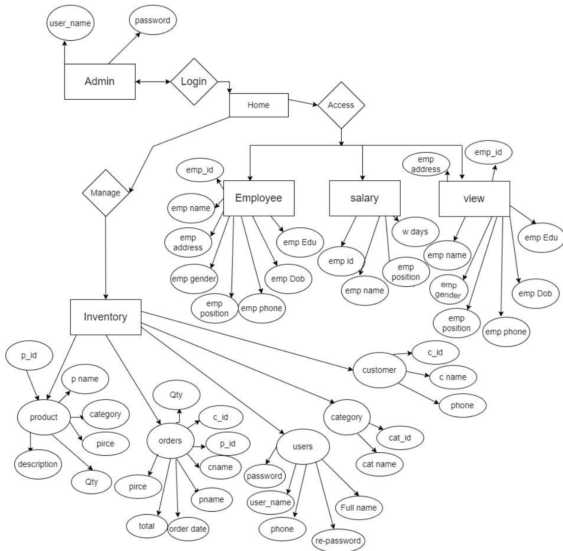
Fig3.2.1 ER diagram of inventory management system
