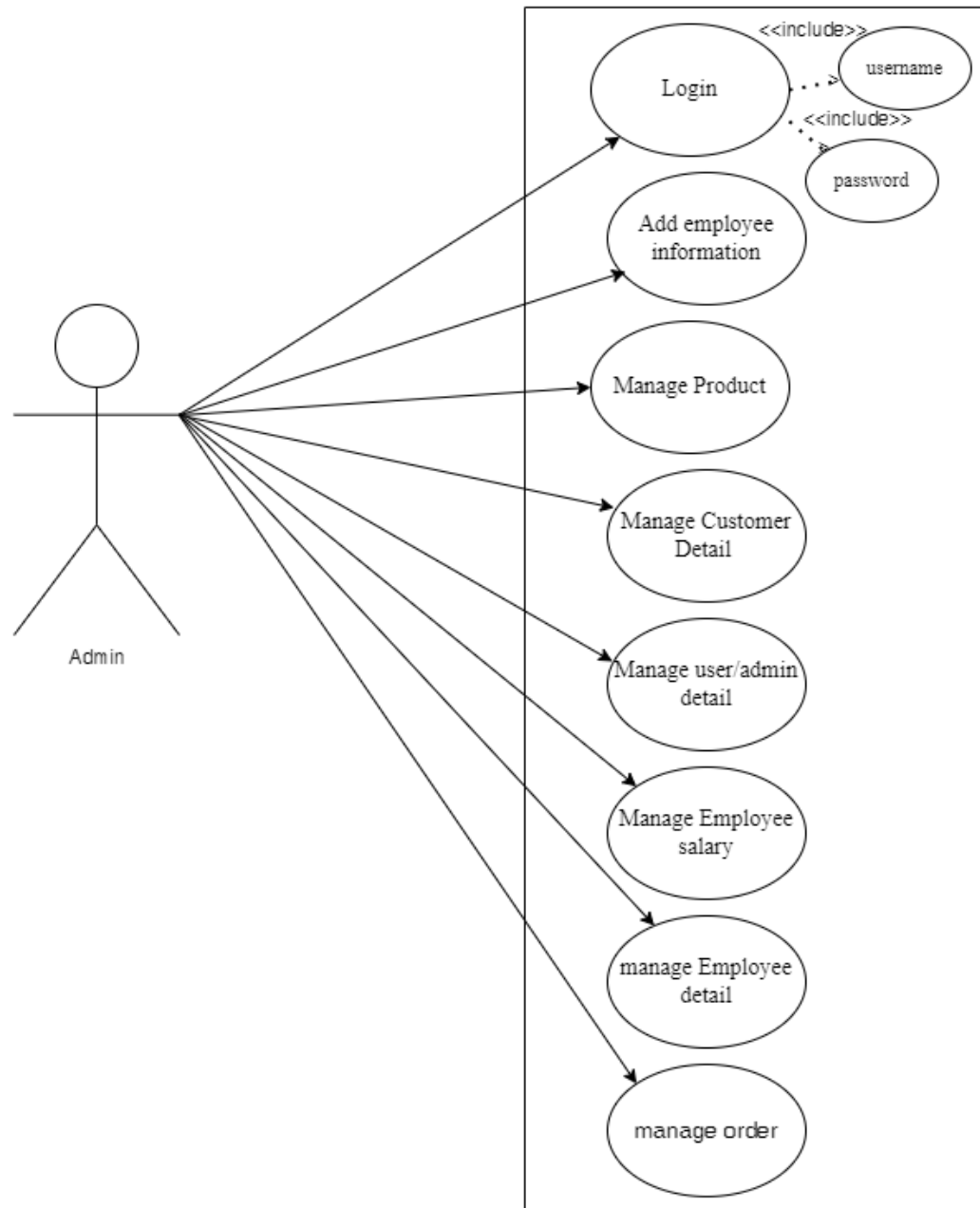
Fig 3.3.1 Use case diagram of inventor management system
