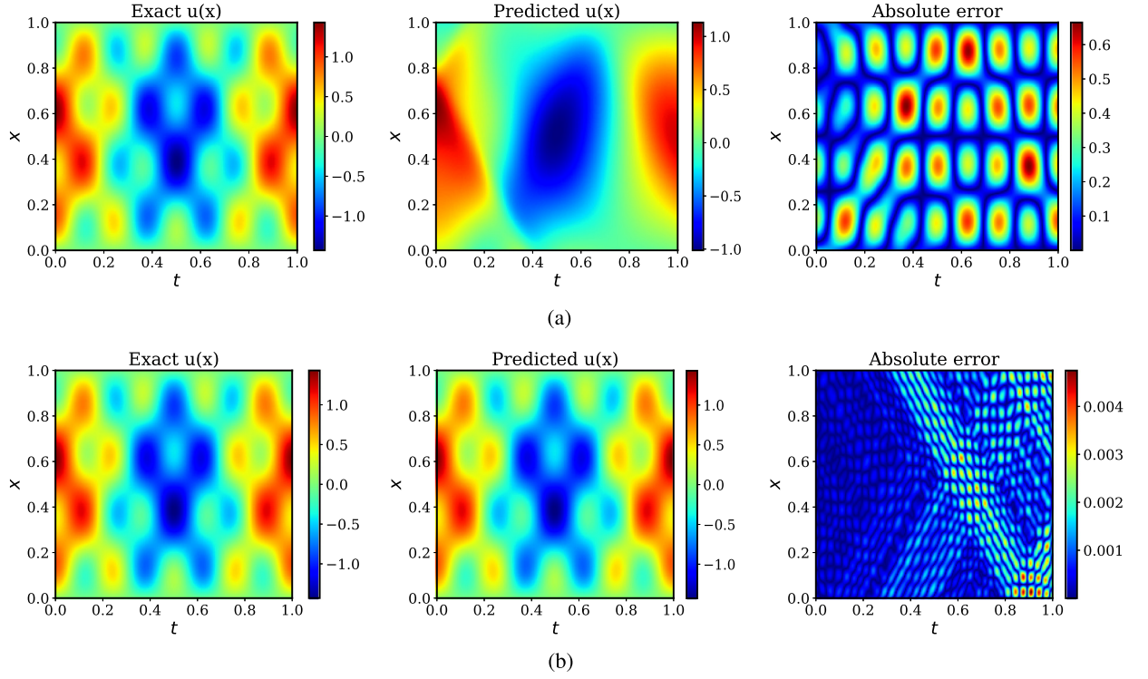
Fig. 6. One-dimensional wave equation: (a) The predicted solution versus the exact solution by training a fully-connected neural network with five hidden layers and 500 neurons per layer using the Adam optimizer with default settings [47] after 80,000 iterations. The relative L^2 error is 4.518e-01 . (b) The predicted solution versus the exact solution by training the same network using Algorithm 1 after 80,000 iterations. The relative L^2 error is 1.728e-03 . (For interpretation of the colors in the figure(s), the reader is referred to the web version of this article.)
