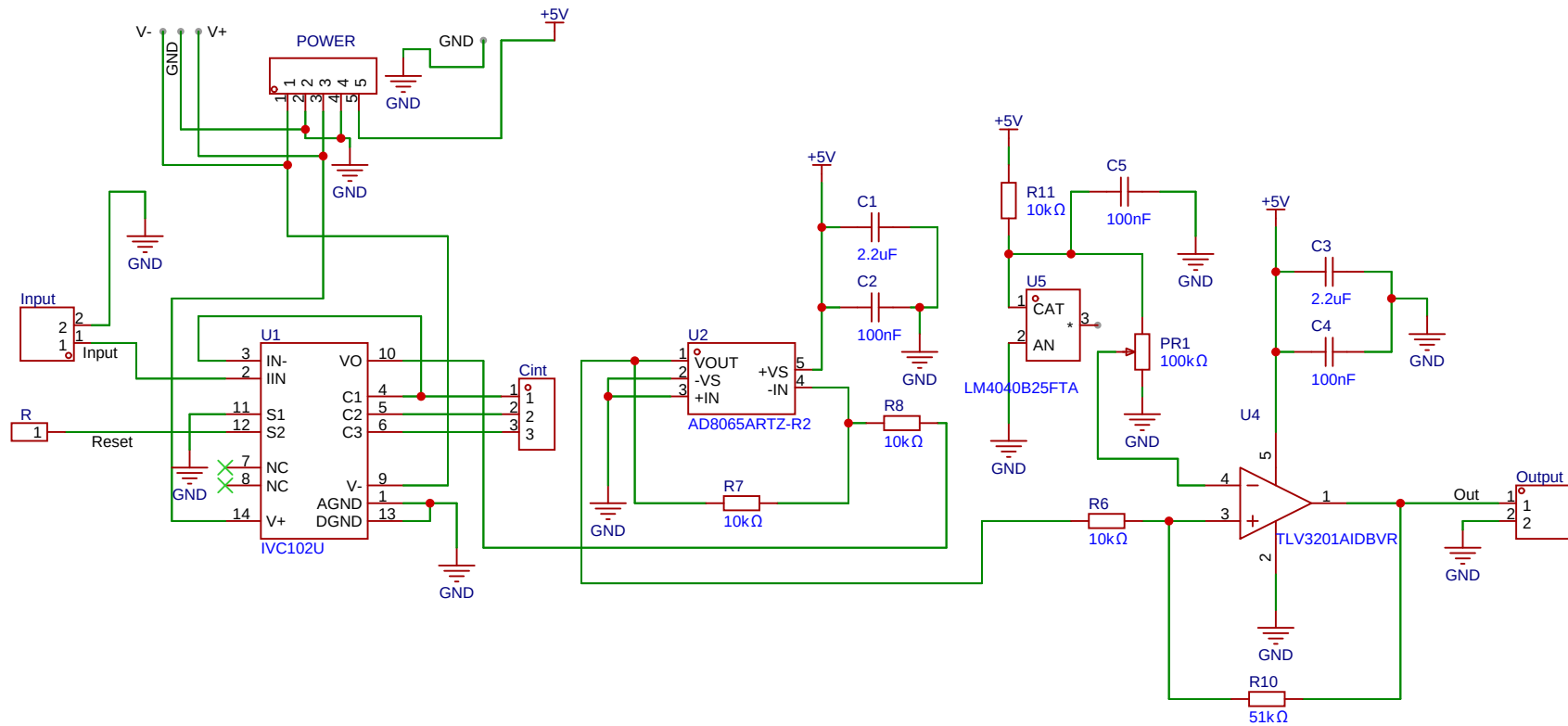
Current Integrator Circuit
