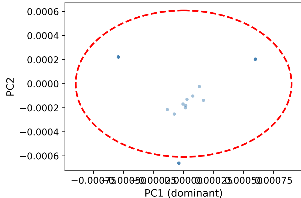
Threshold Neighborhood (projected to PC1-PC2)
