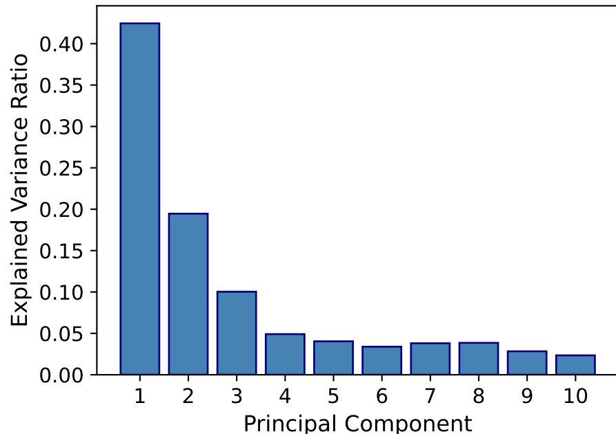
Eigenvalue Spectrum (PC1 = 42% of variance)
