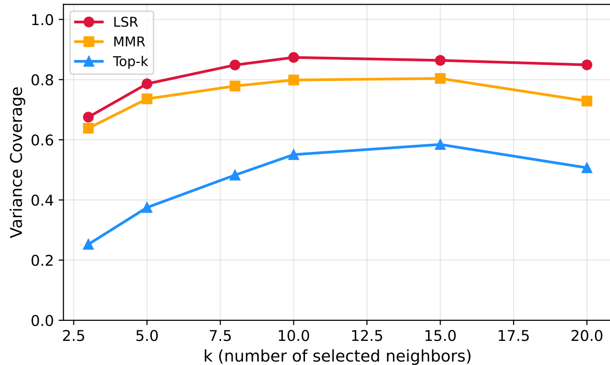
Variance Coverage (Neo4j corpus, 500 queries, \tau=0.85 )
