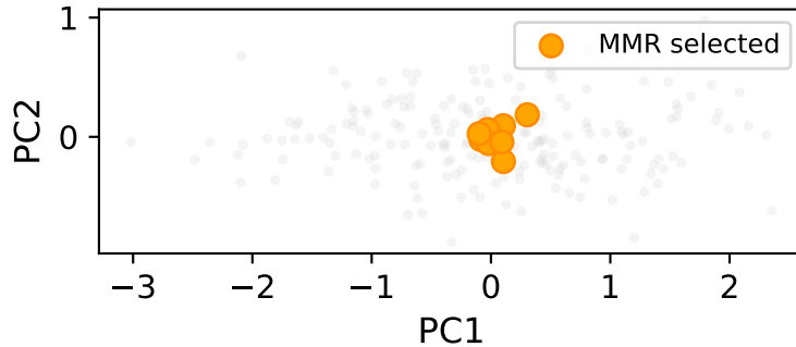
MMR ( \lambda = 0.5 )
