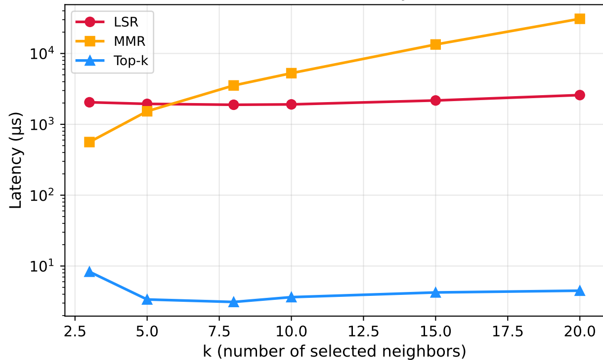
Selection Latency
