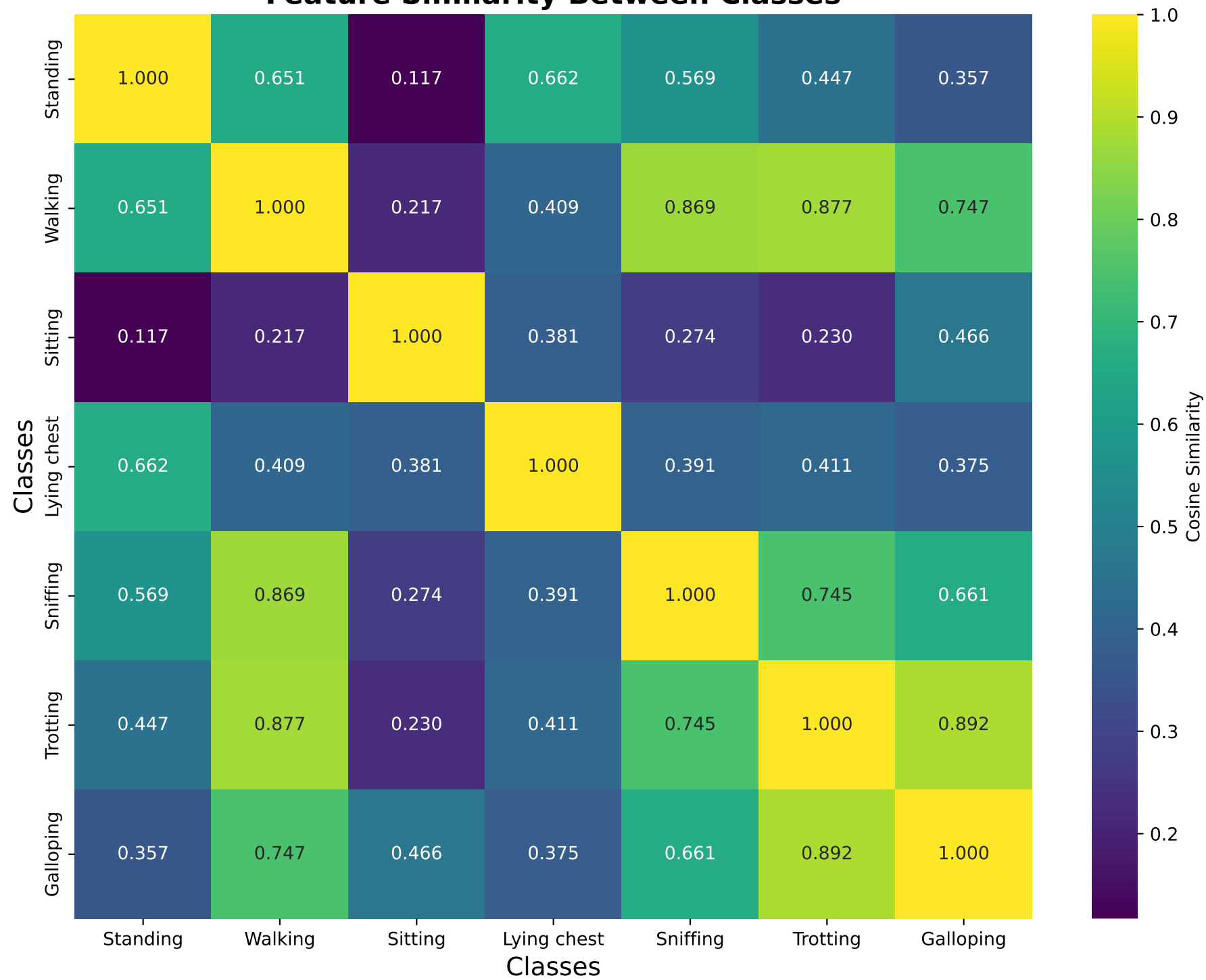
Feature Similarity Between Classes
