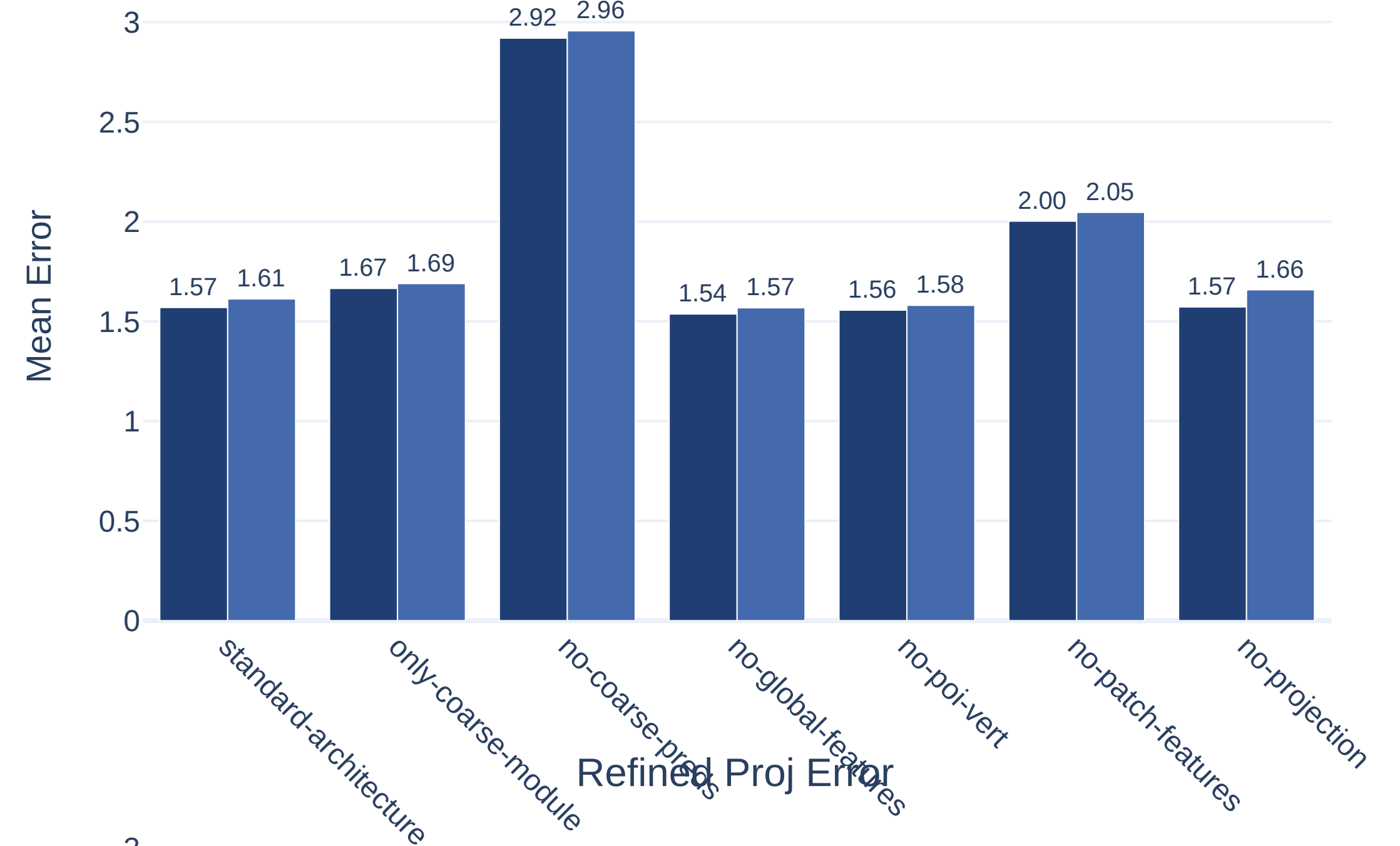
Refined Error
