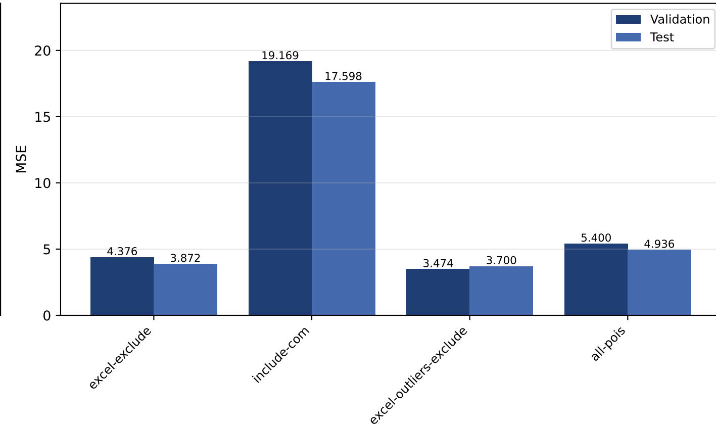
Refined Error
