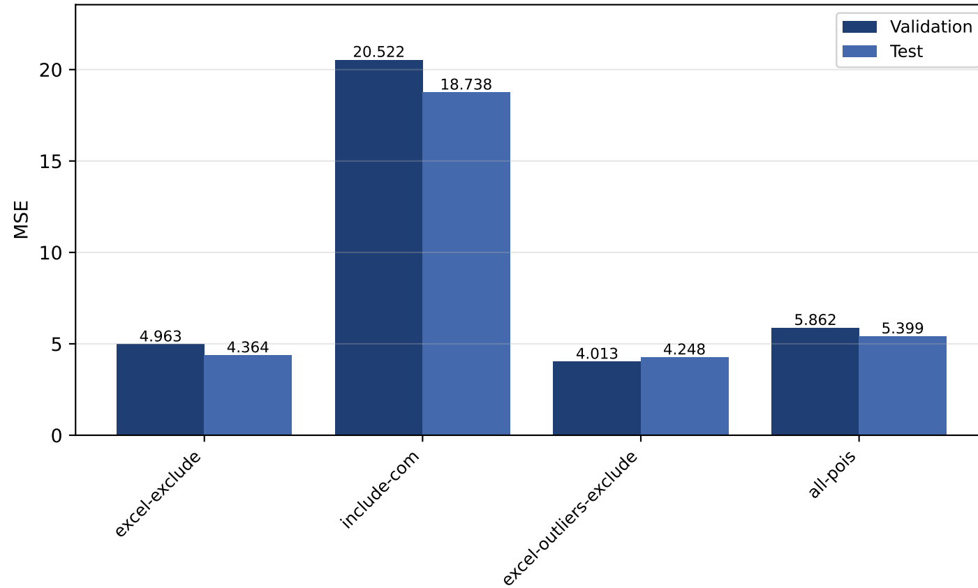
Coarse Error
