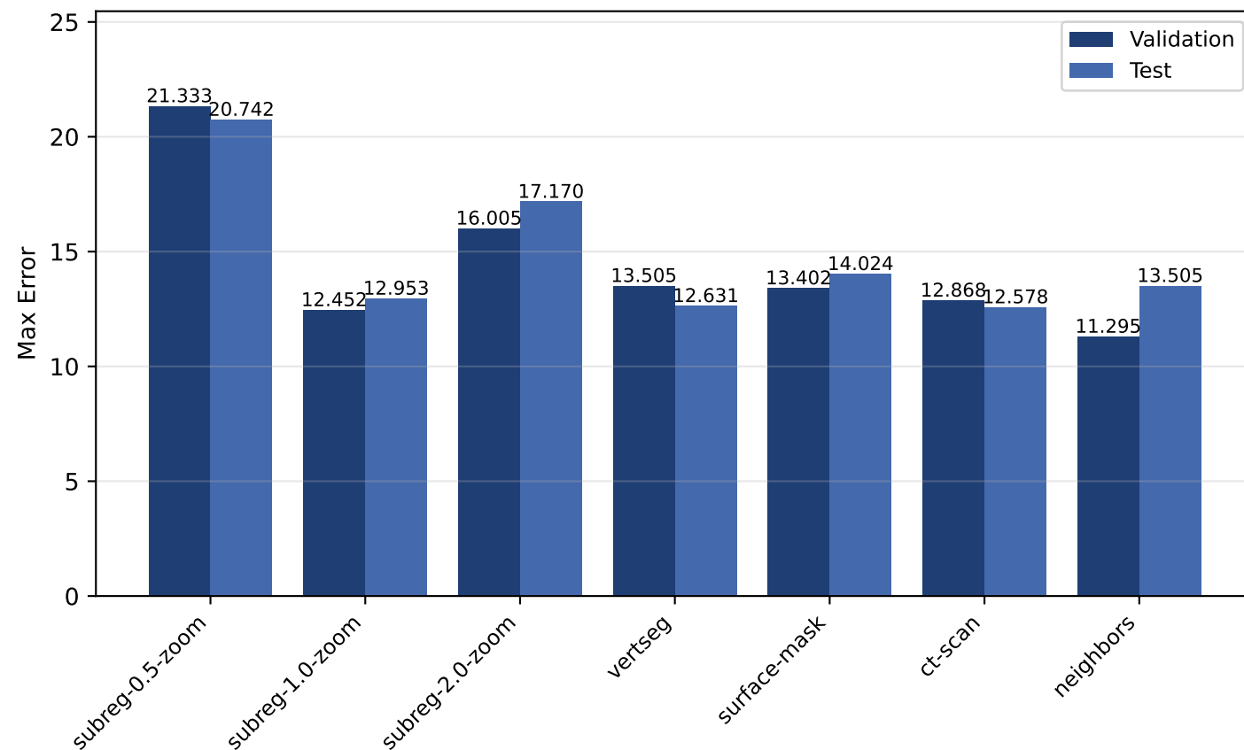
Coarse Error
