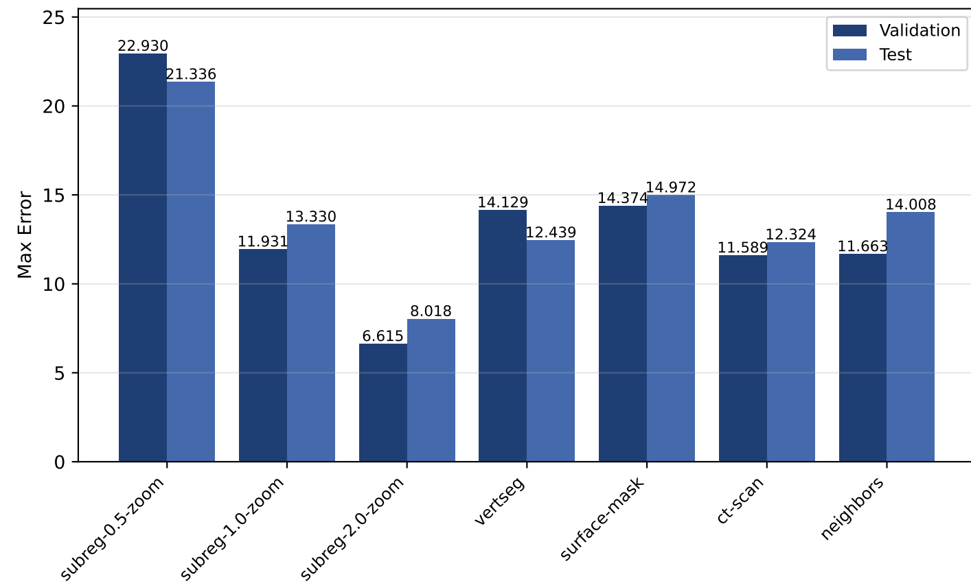
Refined Error
