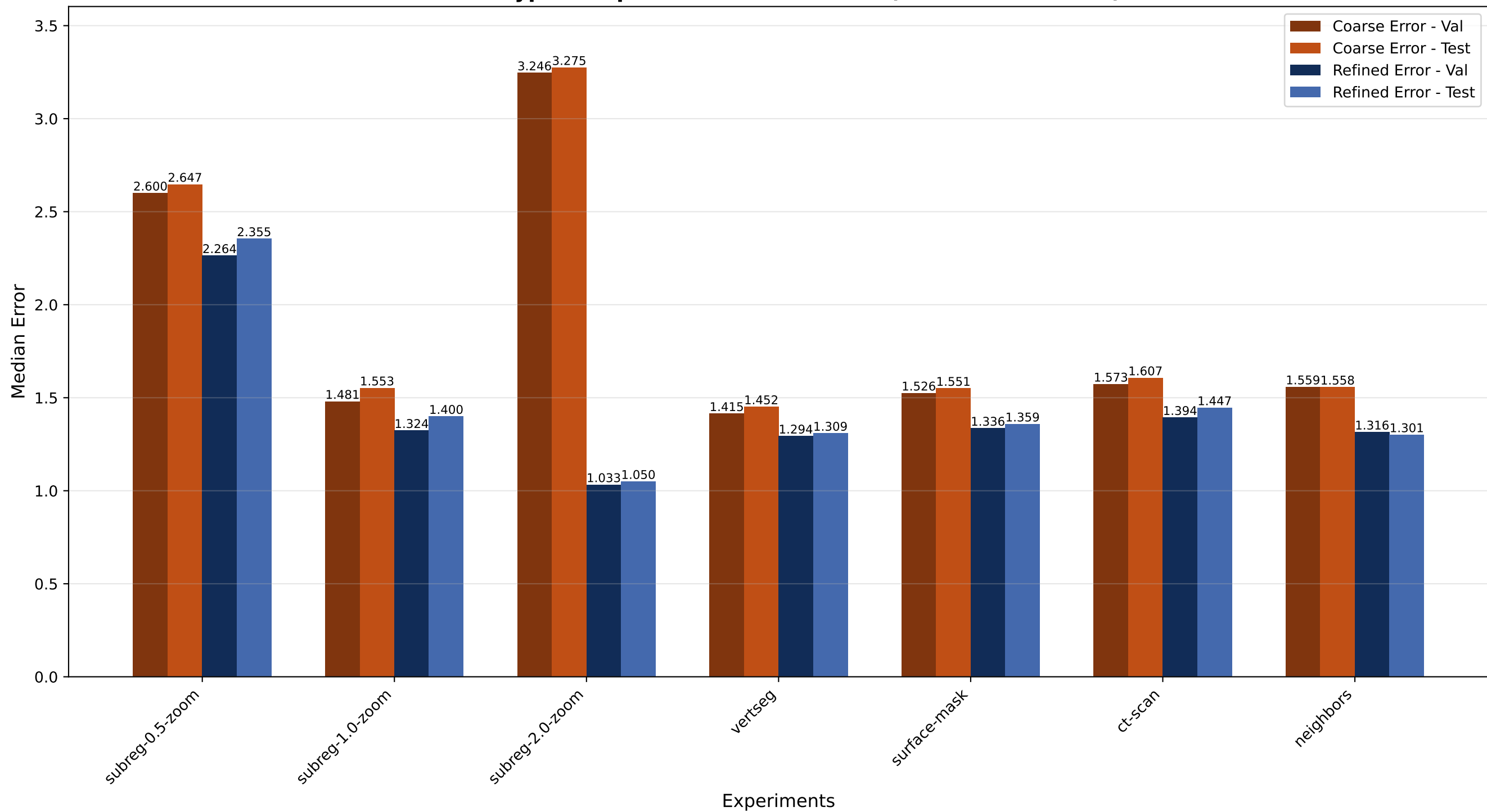
Error Type Comparison - Median Error (Coarse vs Refined)
