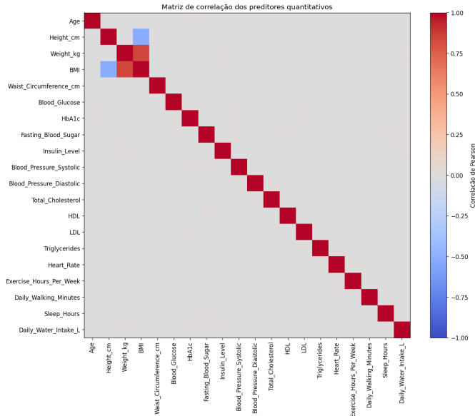
Fig. 4. Pairwise Pearson correlation matrix of the 20 quantitative predictors.
