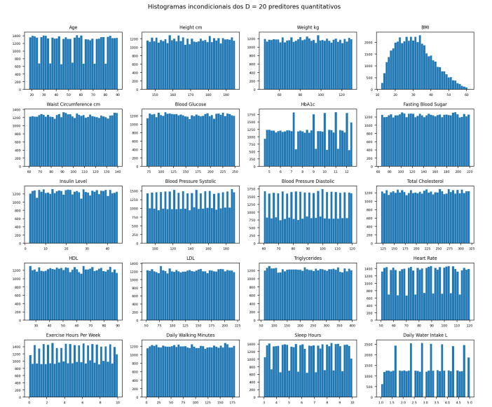
Fig. 1. Unconditional histograms of the 20 quantitative predictors. All but the body mass index are visibly flat-topped.
