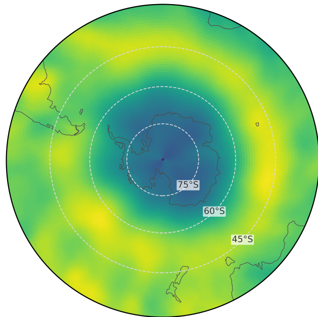
Winds at FL430 (162 hPa), daily means, January 2015-2025 (ERA5)
