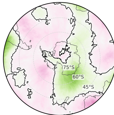
fraction of days with v < 0
