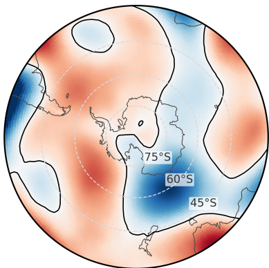
Dec mean v [ \text{m s}^{-1} ] (>0 equatorward)
