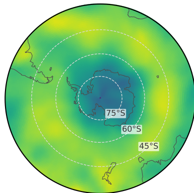
std of daily v [ \text{m s}^{-1} ]
