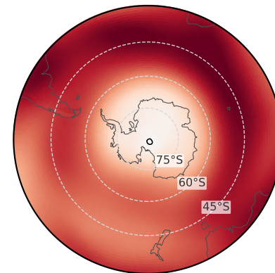
mean u [ \text{m s}^{-1} ]
