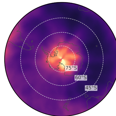
e-folding time \tau [days]
