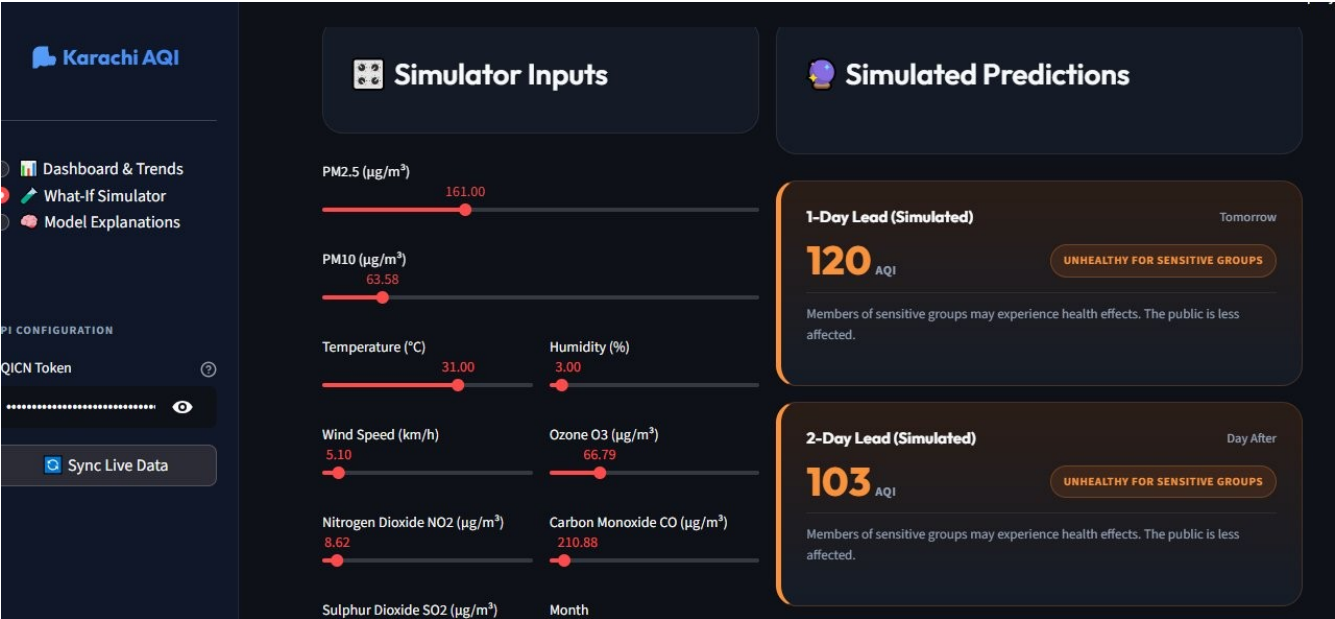
Figure 2: What-If Simulator — Inputs & Simulated Predictions (Jun 06, 2026)
