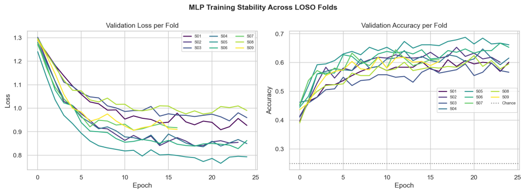
Figure 16: Validation loss and accuracy trajectories for the MLP across all nine LOSO folds, illustrating training stability across subjects.
