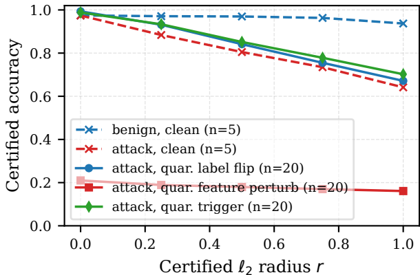
CIC-UNSW-NB15, \sigma = 0.5 , N = 200
