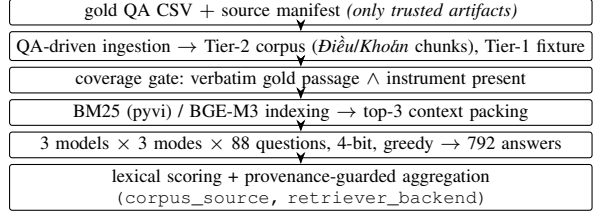
Fig. 1. The RegRAG-VN pipeline. Every record crossing a component boundary carries the corpus_source and retriever_backend tags enforced by the aggregation guard; the coverage gate excludes a question rather than let it generate a false hallucination label.
