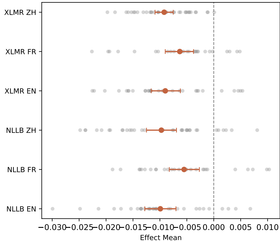
H1 Semantic FFN Preference
